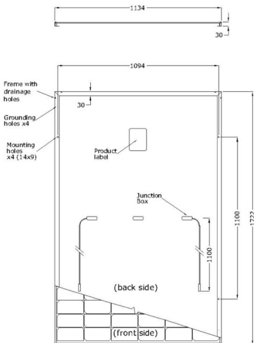
Fig. 5: Mechanical drawing of the FU XXX M / MV SILK® PLUS (108 half-cut cells) module showing the mounting holes, the drainage holes, and the ground connection holes.
