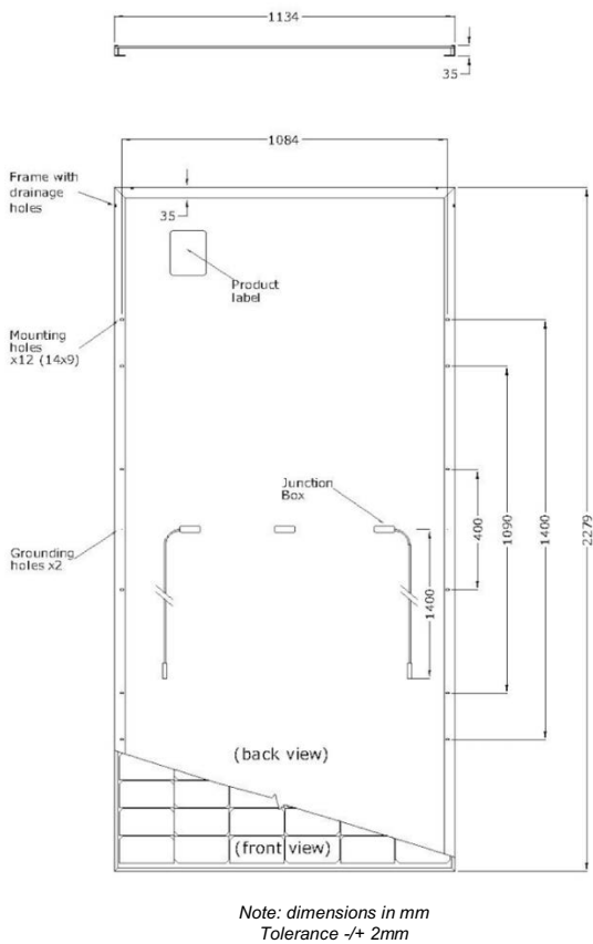
Fig. 6: Mechanical drawing of the FU XXX M / MV SILK ® PLUS (144 half-cut cells) module showing the mounting holes, the drainage holes, and the ground connection holes.
